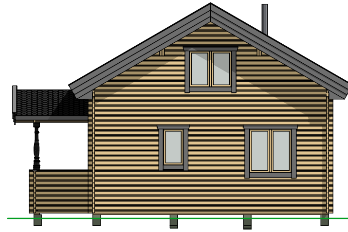
A2 Right view 1:100
