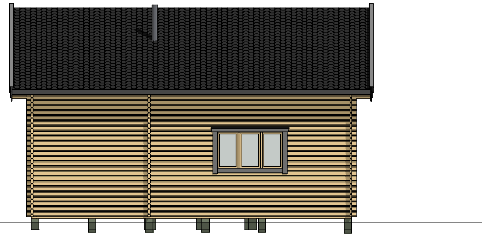
A3 Rear view 1:100
